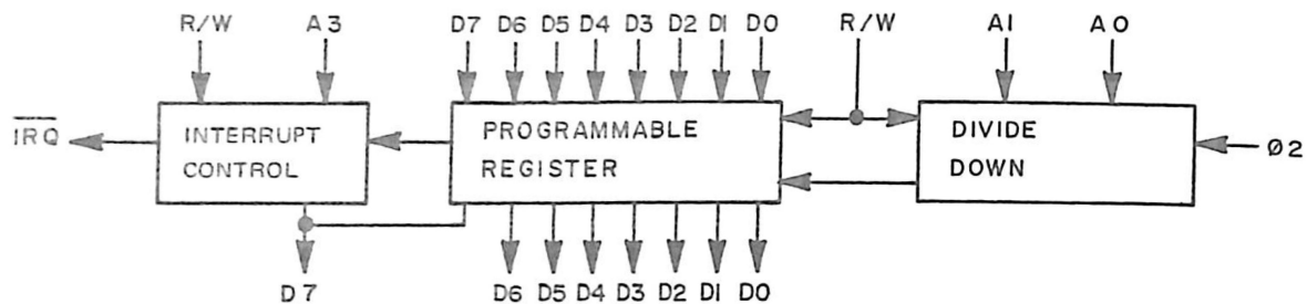
BASIC ELEMENTS OF INTERVAL TIMER - Figure 4
